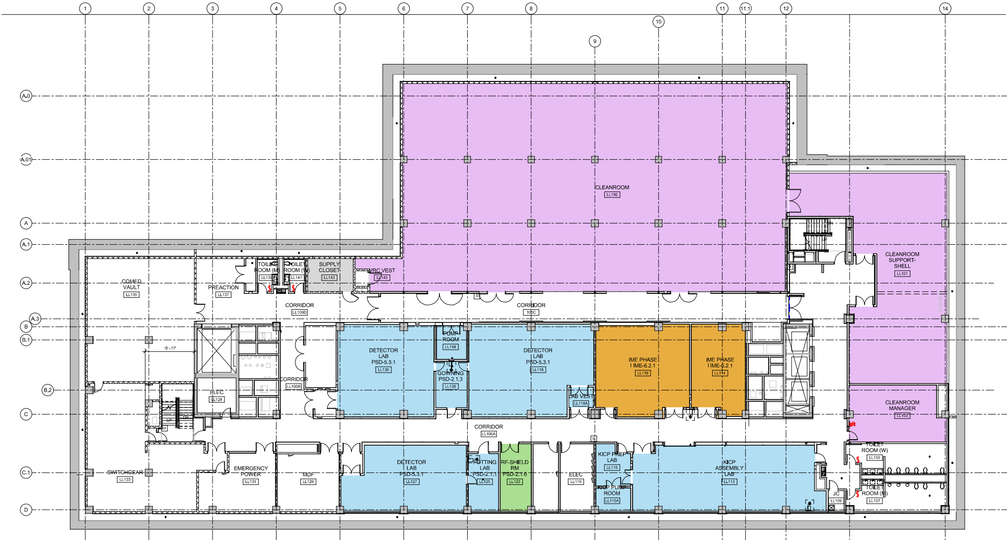
1 LOWER LEVEL 1 FLOOR PLAN 3/32" = 1'-0"
